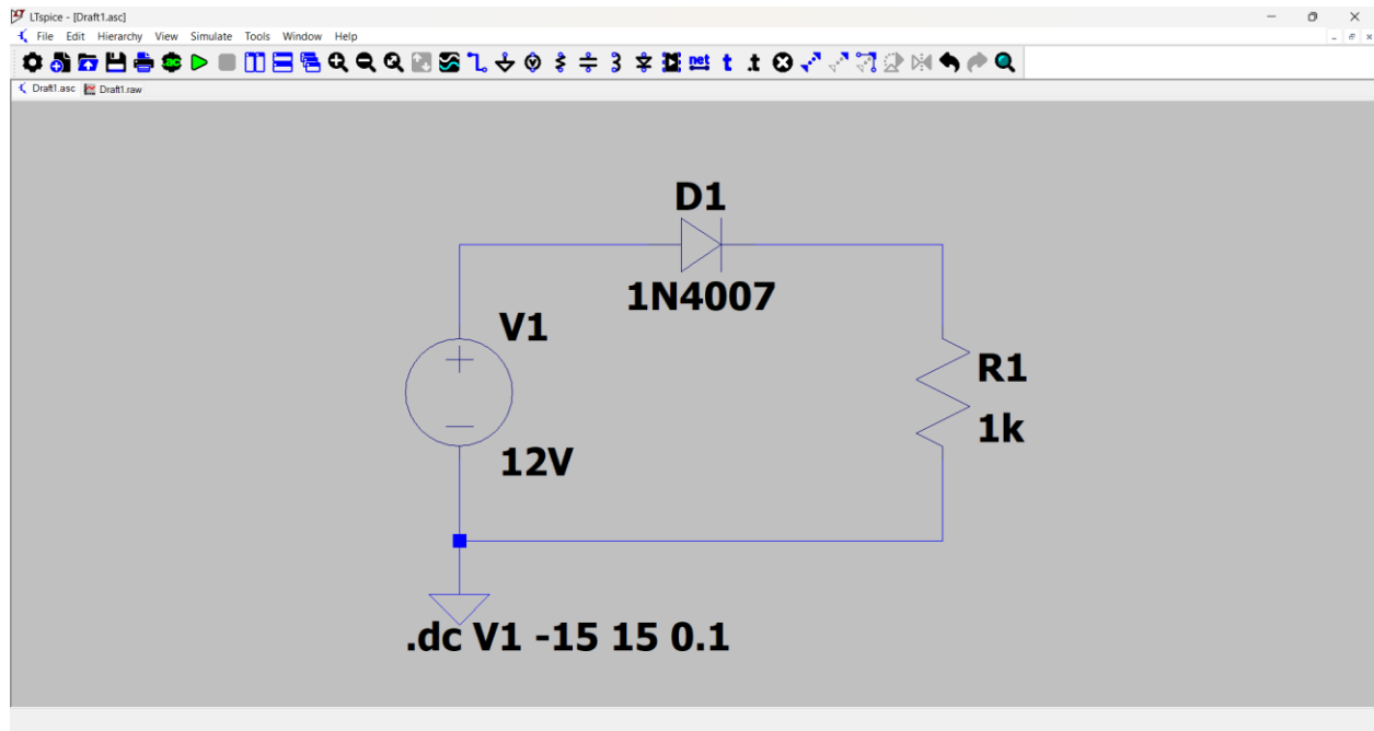
Figure 1: Diode Selection for a Real Application
